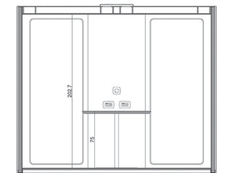
BUSYPOD XLarge plan section
